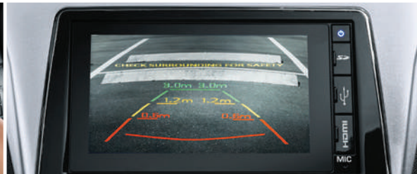
Reverse Camera
